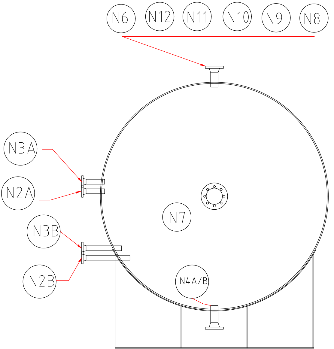
SIDE VIEW B-B
