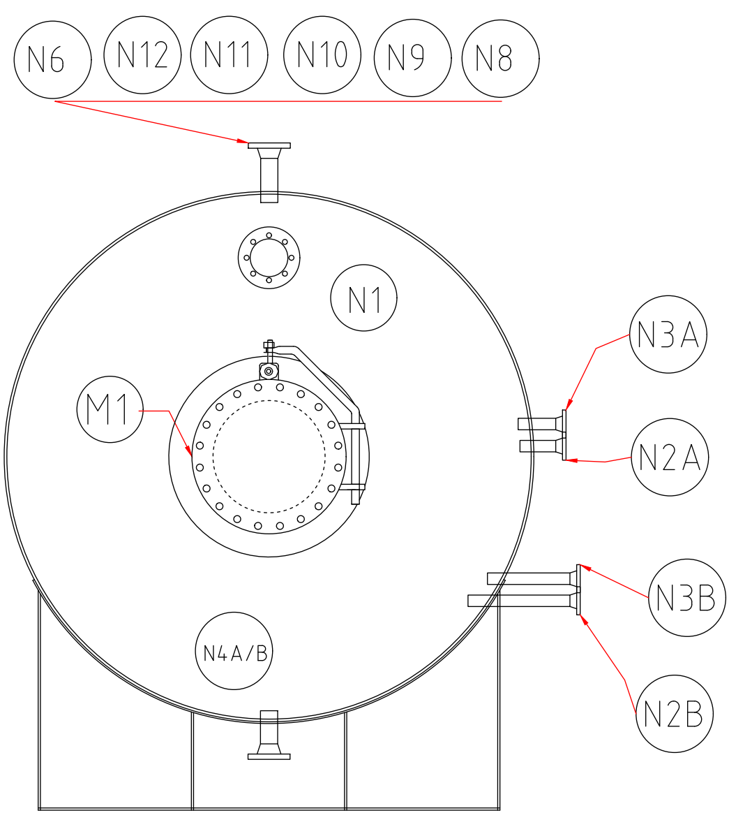
SIDE VIEW C-C
